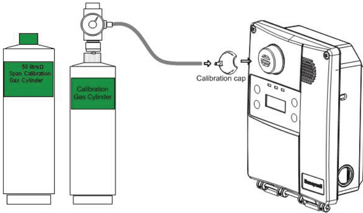
Figure 6. Calibration Setup
