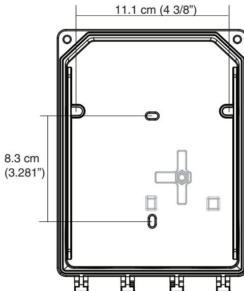
Figure 1. Unit Dimensions
