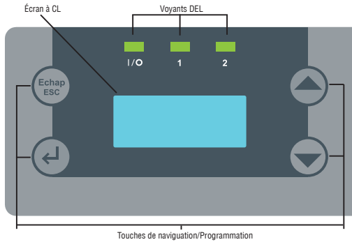
Illustration 4. ACL E 3 Point
