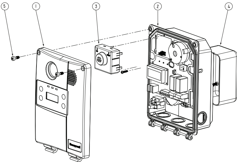
Figure 7. Parts of the E 3 Point
